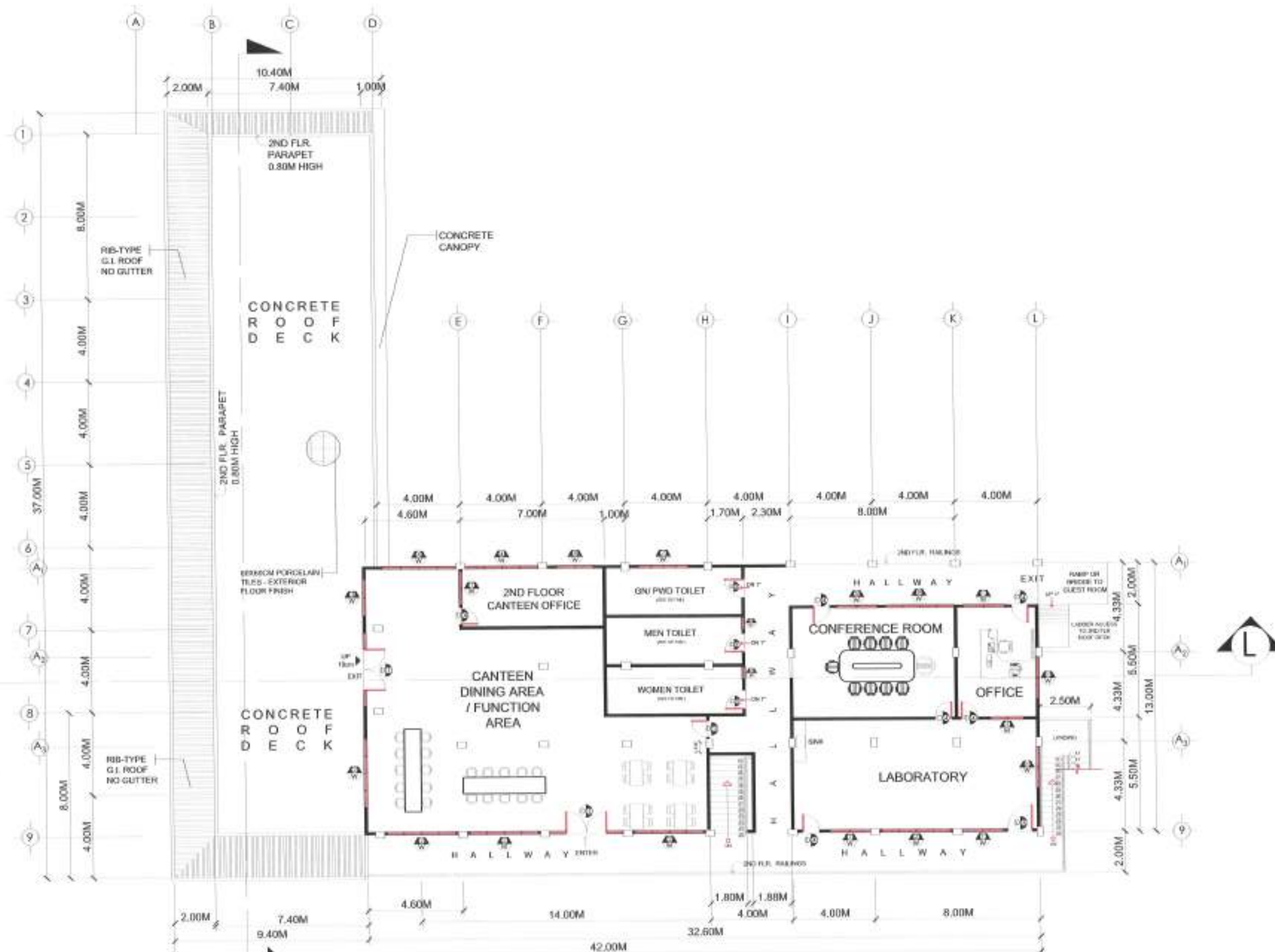
1 SECOND FLOOR PLAN A - 3 SCALE: 1:200 MTS.
