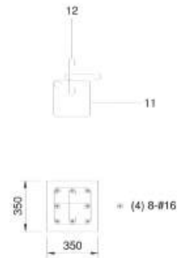
SECTION 3-3 (C25) (SCALE 1:25)
