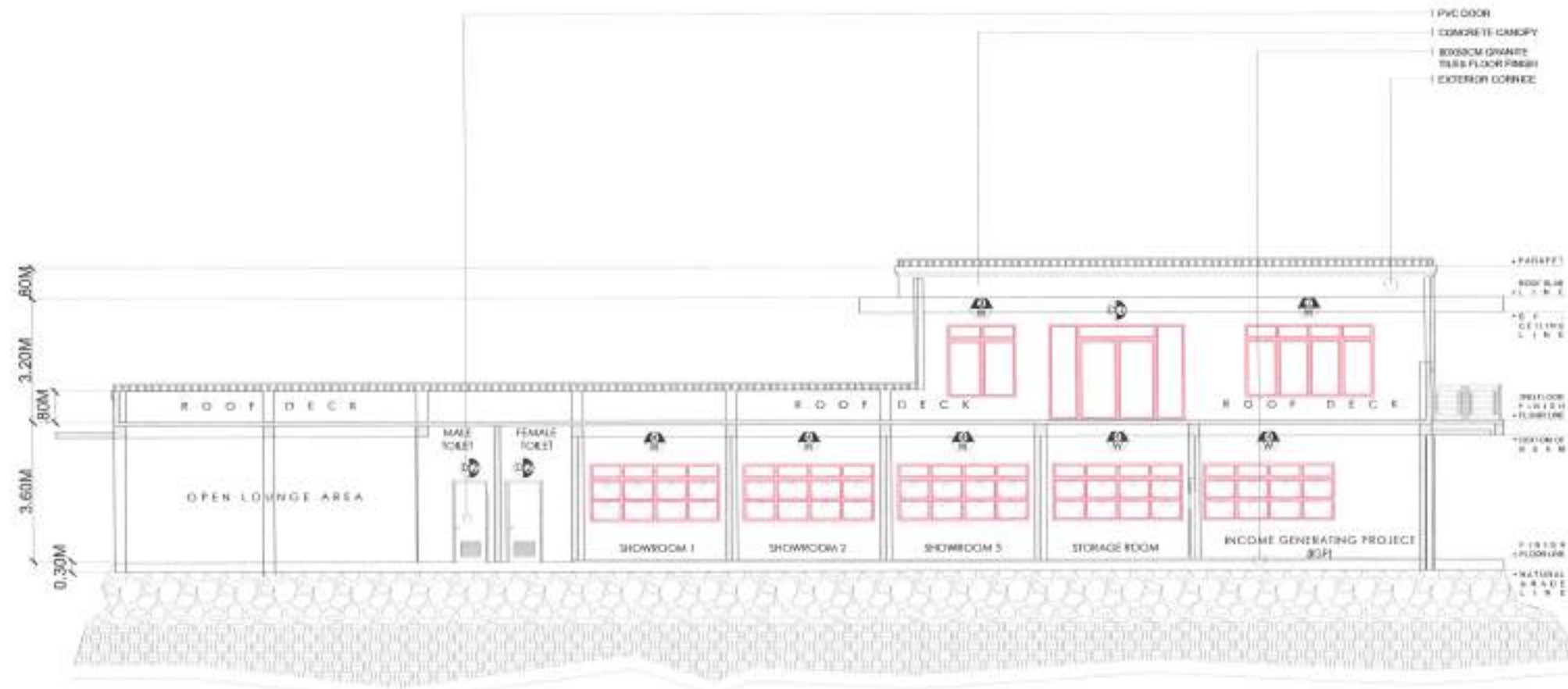
1 CROSS SECTION A-10 SCALE: 1:200 MTS.
