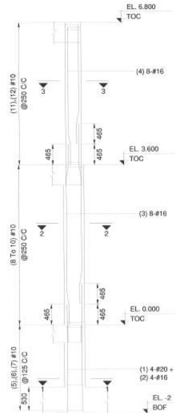
DETAIL OF COLUMN C25 (SCALE 1:50)
