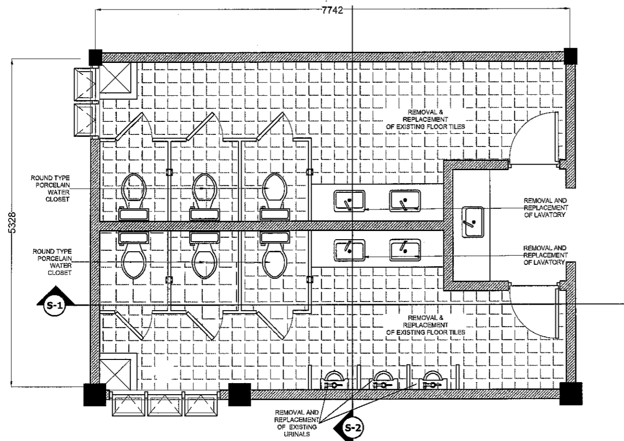
1 COMMON CR AT SECOND FLOOR A-3 SCALE 1:30 MTS.
