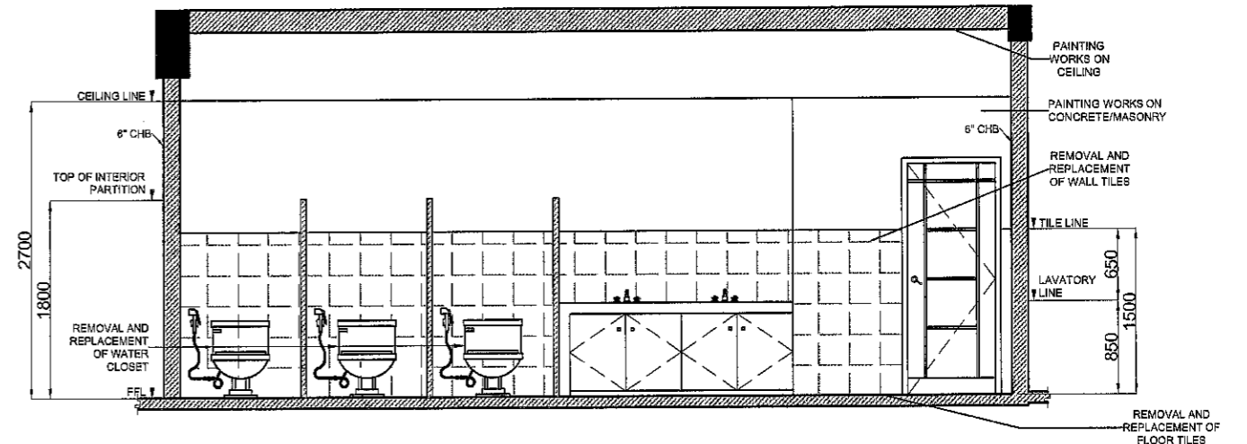
2 SECTION - 1 PLAN A-3 SCALE 1:30 MTS.
