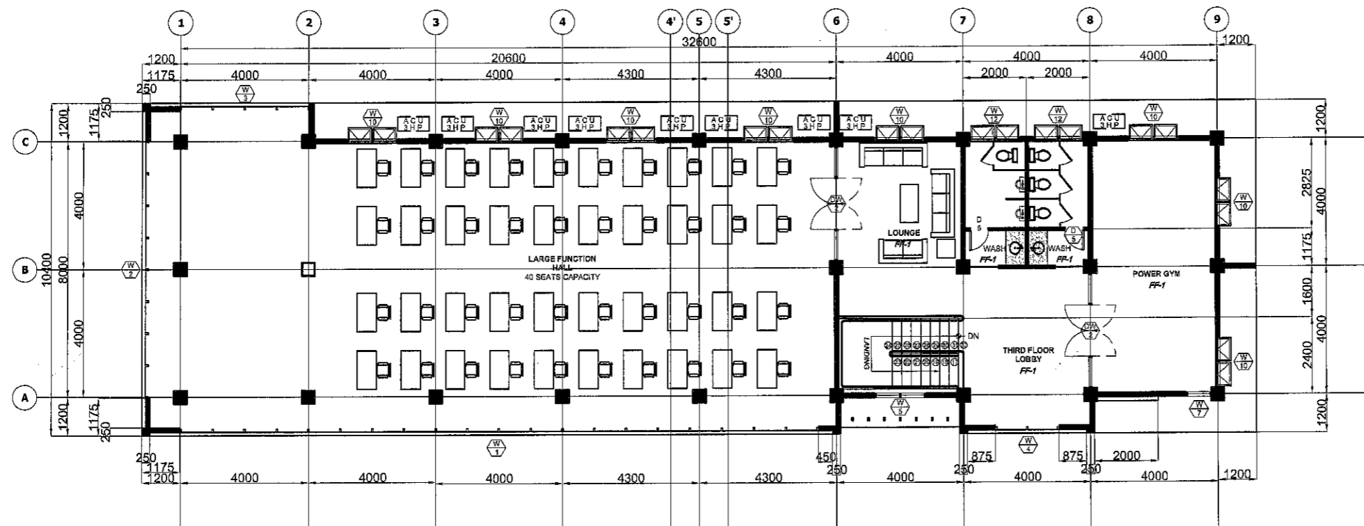
1 MULTI-PURPOSE BUILDING THIRD FLOOR PLAN A-4 SCALE 1:80 MTS.
