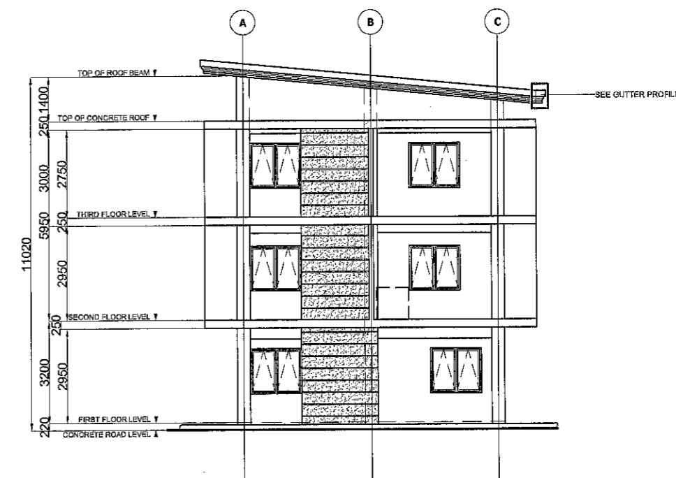
2 MULTI-PURPOSE BUILDING RIGHT ELEVATION A-4 SCALE 1:80 MTS.
