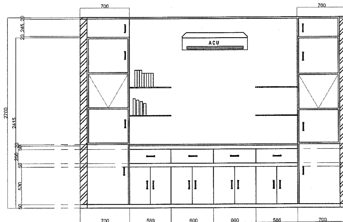
1 DETAIL OF CABINET @ MAINTENANCE SECTION SCALE 1:15 MTS.
