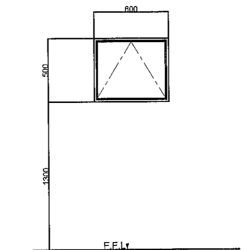
4 WINDOW SCHEDULE SCALE 1:20 MTS.
