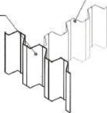
SHEET PILE AT INTERMEDIATE WALL (ISOMETRIC VIEW)
