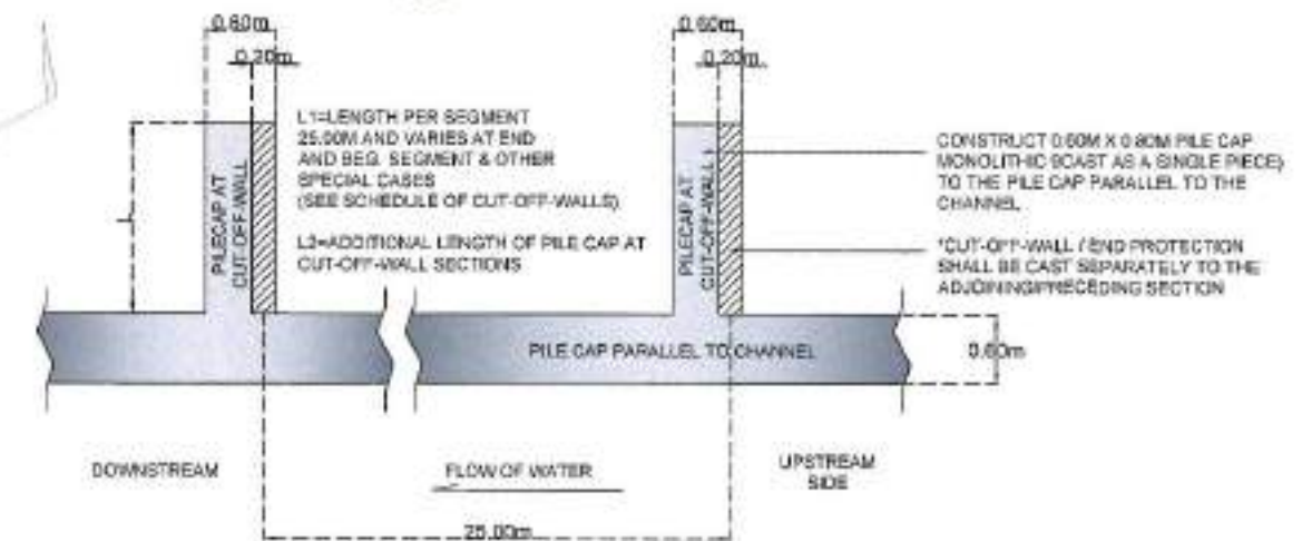
PILE CAP LAYOUT AT CUT-OFF-WALL SECTION
