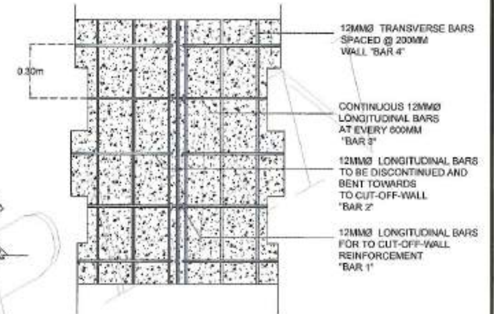
LONGITUDINAL VIEW OF CONCRETE FACING AT CUT-OFF-WALL SECTION
