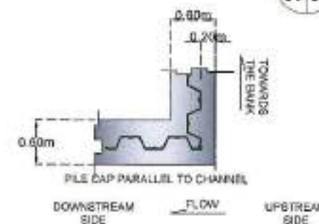
SHEET PILE LAYOUT AT END WALL SECTION
