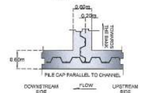
SHEET PILE LAYOUT AT CUT-OFF-WALL SECTION
