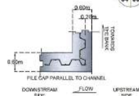
SHEET PILE LAYOUT AT END WALL SECTION
