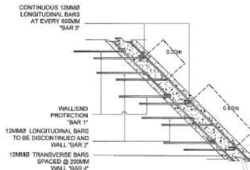
SECTION VIEW OF CONCRETE FACING AT CUT-OFF-WALL SECTION
