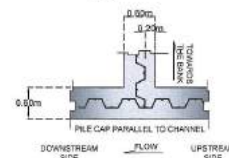
SHEET PILE LAYOUT AT CUT-OFF-WALL SECTION
