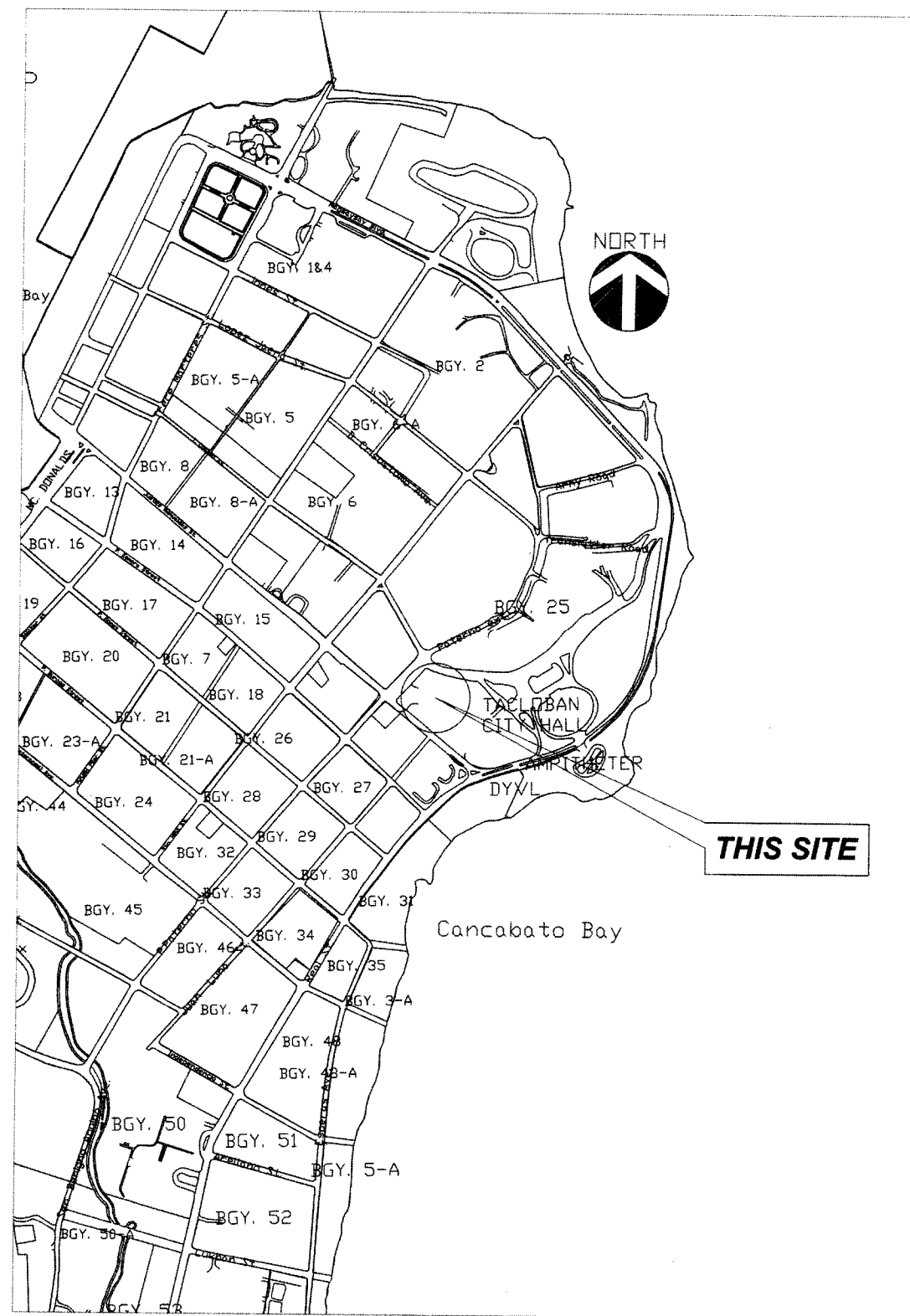
VICINITY MAP
