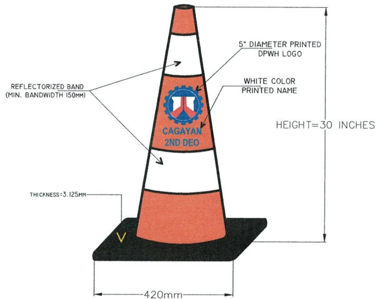
RUBBERIZED TRAFFIC CONE W/ REFLECTORIZED BAND
