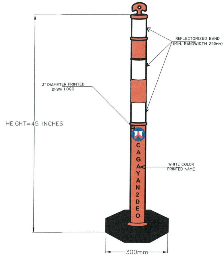
PLASTIC PVC T-BOLLARD W/ RUBBERIZED BASE AND REFLECTORIZED BAND
