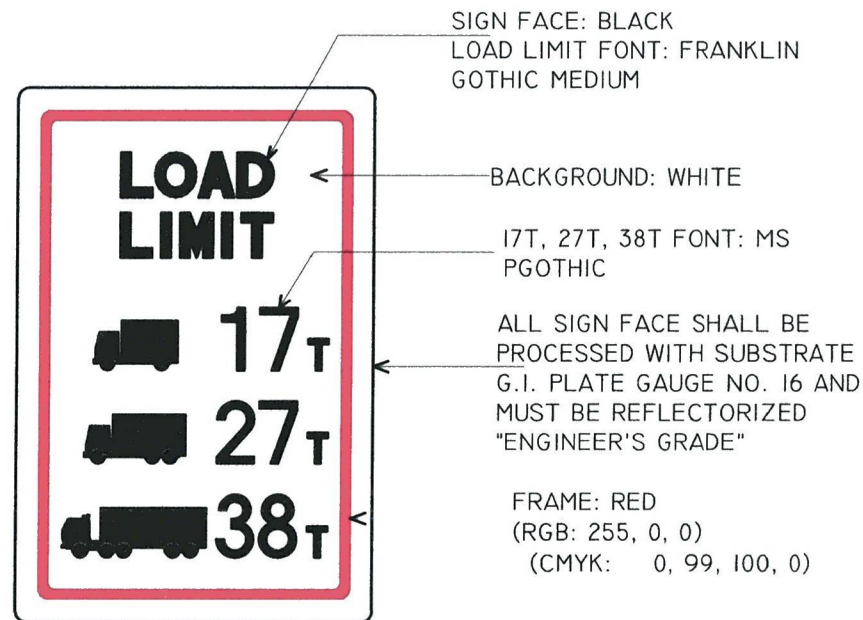
DETAIL OF LOAD LIMIT SIGN FACE SCALE 1:100 METERS
