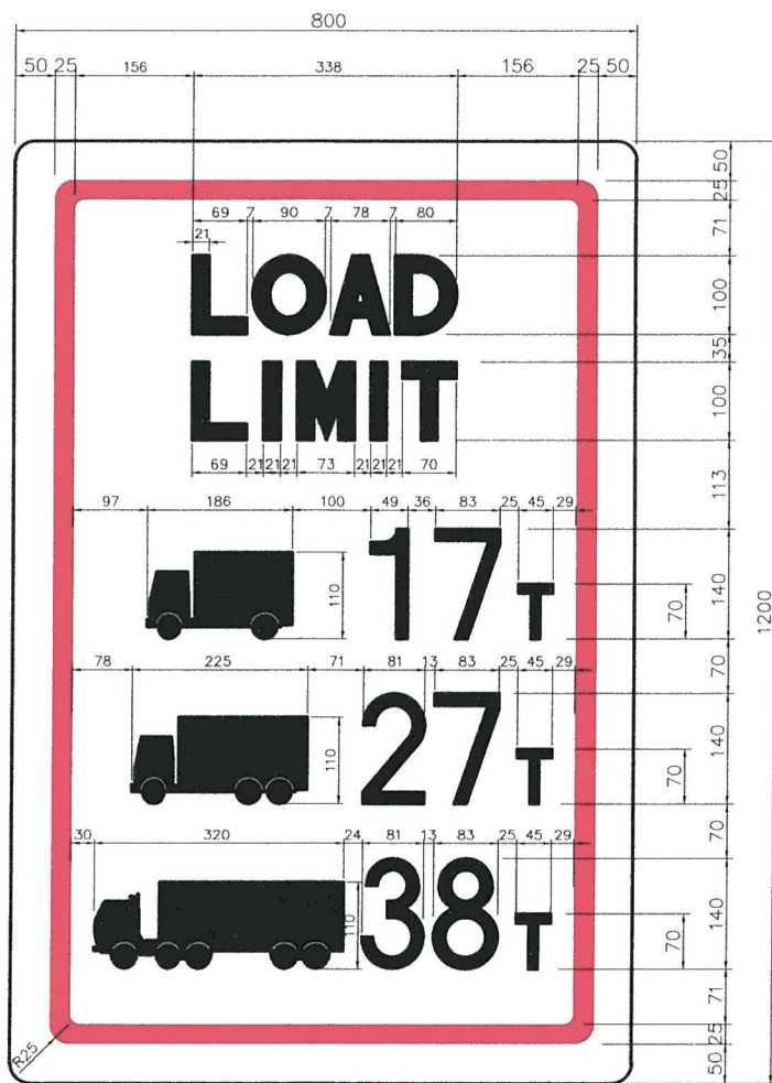
DETAIL OF SERIES 120DN LETTERS & NUMERICAL DIMENSIONS SCALE 1:50 METERS
