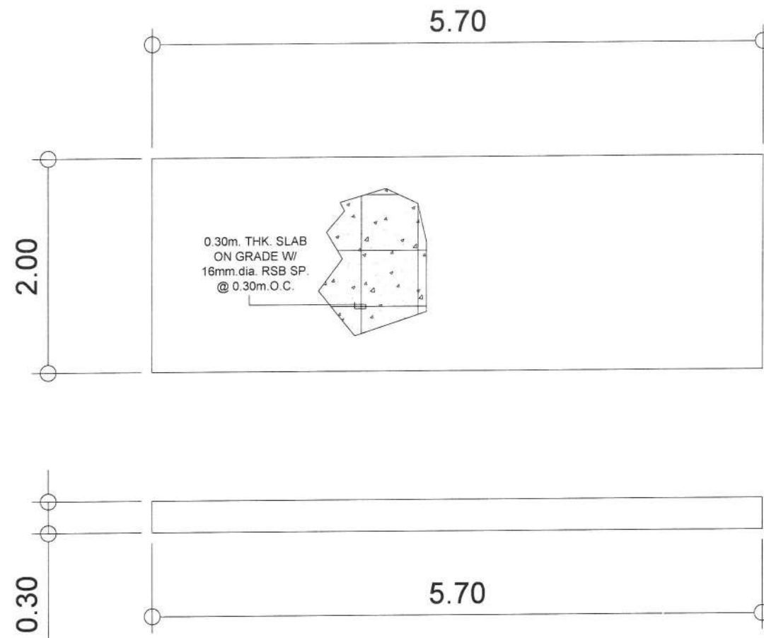
GROUND FLOOR PLAN PLATFORM DETAILS SCALE 1:50 MTS
