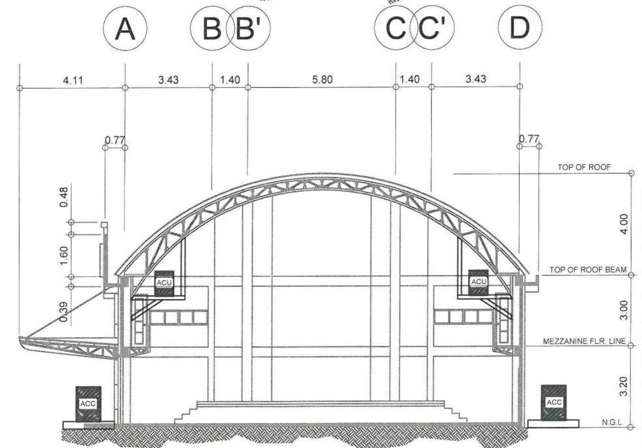
CROSS SECTION SCALE 1:150 MTS
